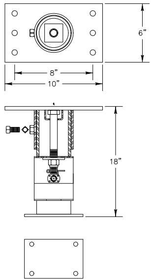
Vertical Mounting Bracket (Non-Oscillating)
